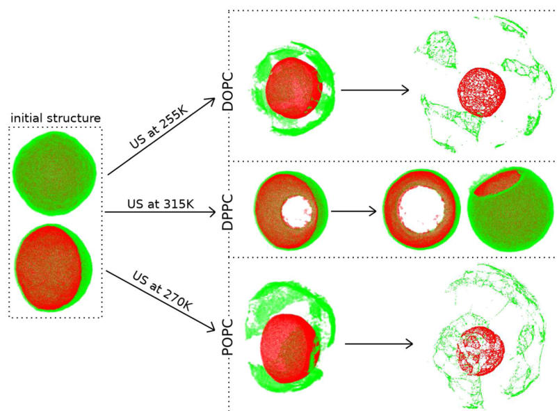
Figure 5. Initial structure (left) and snapshots of three liposomes DOPC, DPPC, and POPC obtained from simulations at temperatures just above (315 K for DPPC) or just below (255 and 270 K for DOPC and POPC, respectively) the phase transition temperatures. The ultrasound intensities of 720, 500, and 650 bar are used for the DOPC, DPPC, and POPC simulations, respectively. The frequency of 20 MHz is used in all simulations. The inner and outer leaflets are shown in red and green, respectively.
