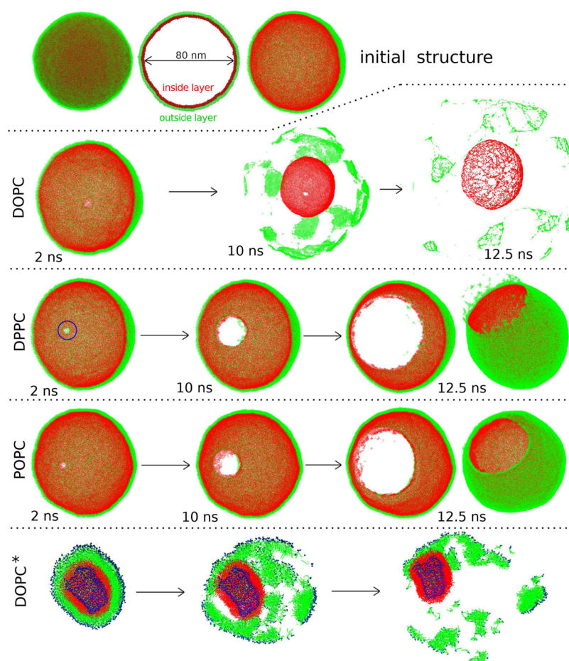
Figure 1. (Top) Initial structure of the DPPC liposome. (Middle) The selected snapshots at various moments of the coarse-grained DOPC, DPPC, and POPC liposomes. (Bottom) The selected snapshots of the all-atom DOPC liposome (denoted as DOPC*). Shown are results obtained from simulations using the ultrasound frequency of 20 MHz and intensity of 640 bar for the DOPC and DOPC* liposomes, 550 bar for the DPPC liposome, and 580 bar for the POPC liposome. For all liposomes, the inner and outer leaflets are colored in red and green, respectively.
