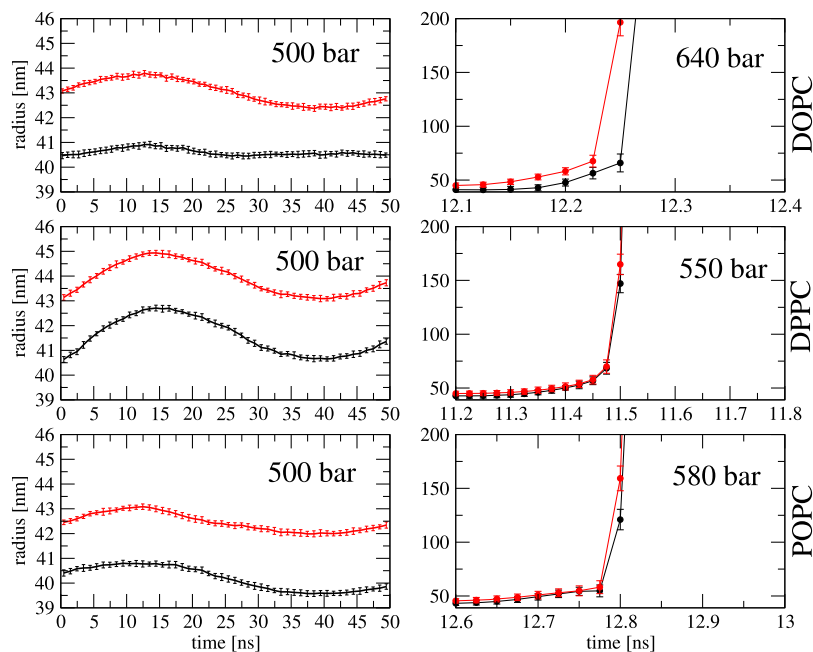
Figure 3. Time evolution of the inner (black lines) and outer (red lines) radii of the three liposomes. All liposomes are stable up to an ultrasound intensity of 500 bar (left panels) but undergo large changes at higher intensities (right panels). The error bars are estimated from five trajectories of each system. A frequency of 20 MHz is used in all simulations.
