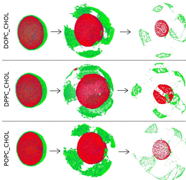
Figure 4. Selected snapshots at t = 0 ns (left), 10 ns (middle), and 12.5 ns (right) of three liposomes DOPC/CHL, DPPC/CHL, and POPC/CHL obtained from simulations using the ultrasound intensity of 670, 630, and 650 bar, respectively. The frequency of 20 MHz is used in all simulations. CHL is shown in blue color. The inner and outer leaflets are shown in red and green, respectively.
