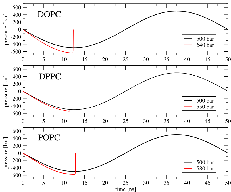
Figure 2. Time evolution of the pressure in the three liposome systems. The pressures of all systems are stably increased and decreased under an ultrasound intensity of 500 bar (black lines). At higher ultrasound intensities, the pressures drop to zero when the ultrasound amplitude is maximum around t \sim \tau/2 = 12.5 ns (red lines), indicating that the systems are exploded. A frequency of 20 MHz is used in all simulations. For clarity, only one ultrasound period is displayed.
